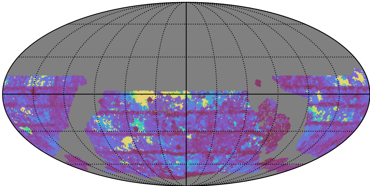
too_elab_r32_d2_gz_v3.4_10yrs WFD z band: Max Inter-Night Gap
