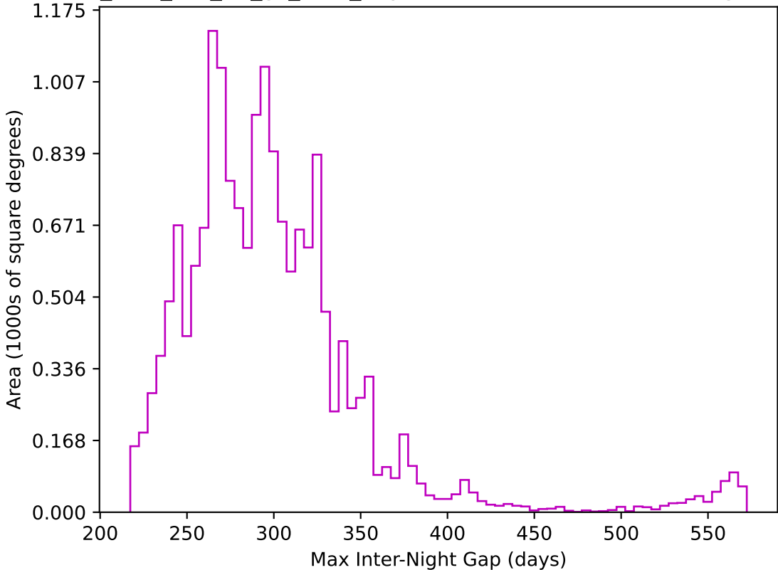
too_elab_r32_d2_gz_v3.4_10yrs WFD z band: Max Inter-Night Gap
