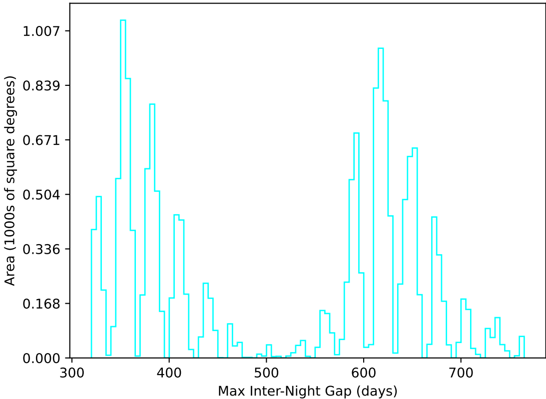
too_elab_r32_d2_gz_v3.4_10yrs WFD u band: Max Inter-Night Gap
