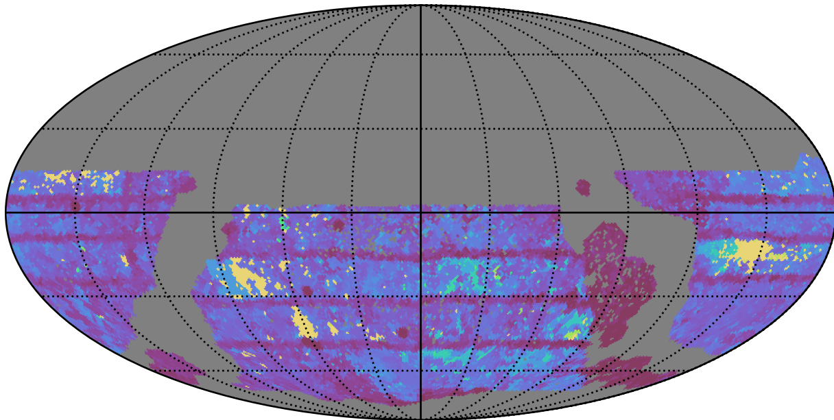
too_elab_r32_d2_gz_v3.4_10yrs WFD r band: Max Inter-Night Gap
