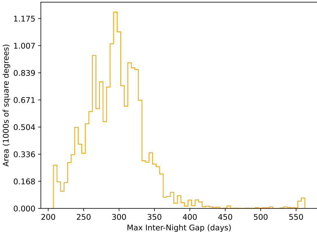
too_elab_r32_d2_gz_v3.4_10yrs WFD r band: Max Inter-Night Gap
