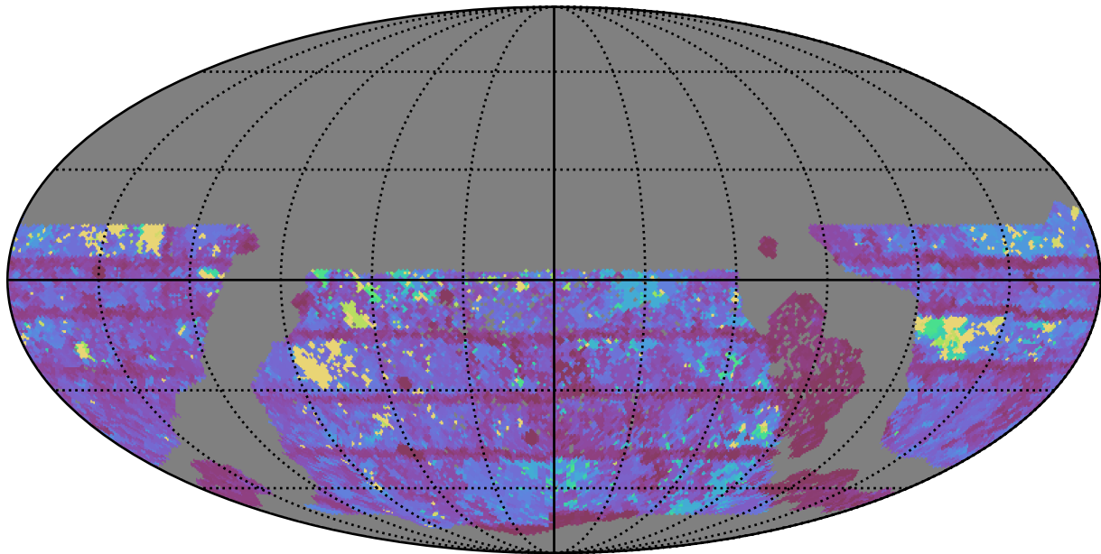
too_elab_r32_d2_gz_v3.4_10yrs WFD i band: Max Inter-Night Gap
