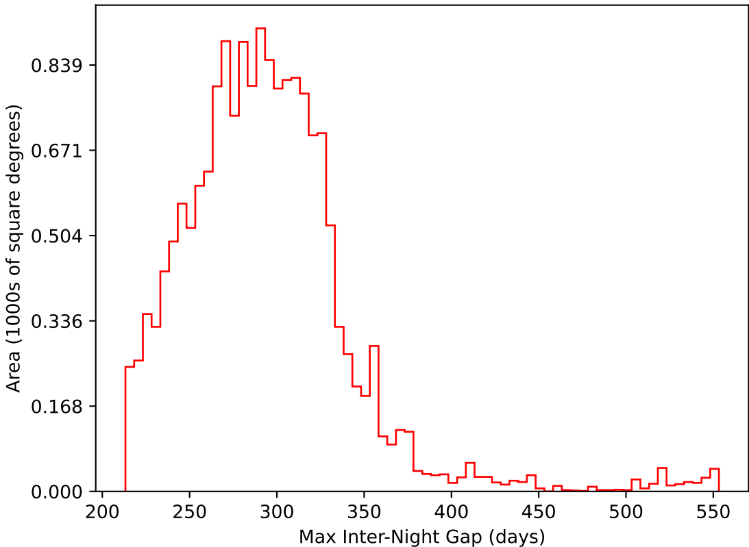
too_elab_r32_d2_gz_v3.4_10yrs WFD i band: Max Inter-Night Gap
