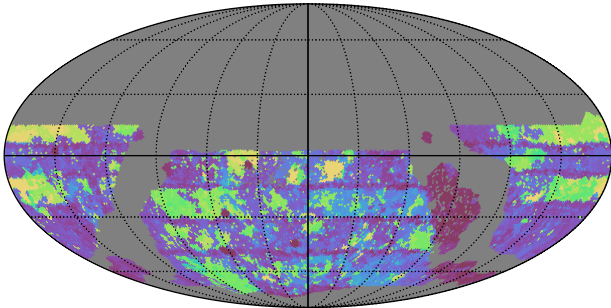
too_elab_r32_d2_gz_v3.4_10yrs WFD g band: Max Inter-Night Gap
