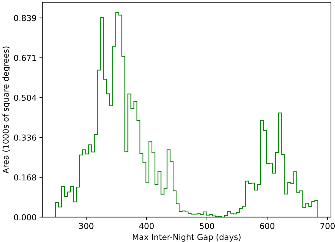
too_elab_r32_d2_gz_v3.4_10yrs WFD g band: Max Inter-Night Gap
