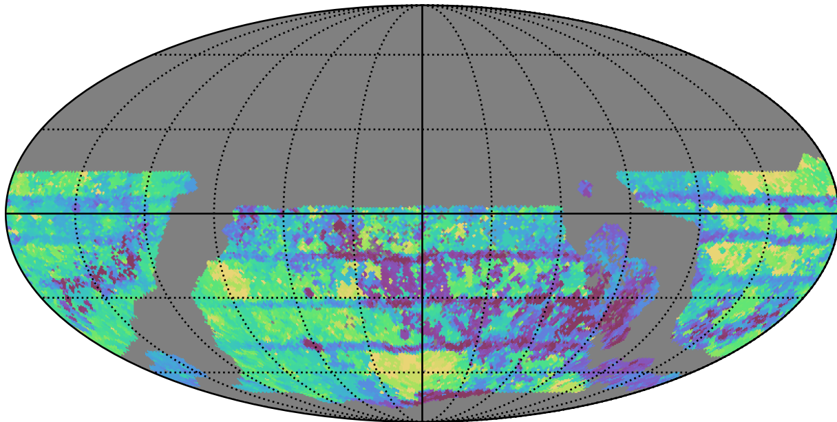
too_elab_r32_d2_gz_v3.4_10yrs WFD all bands: Max Inter-Night Gap
