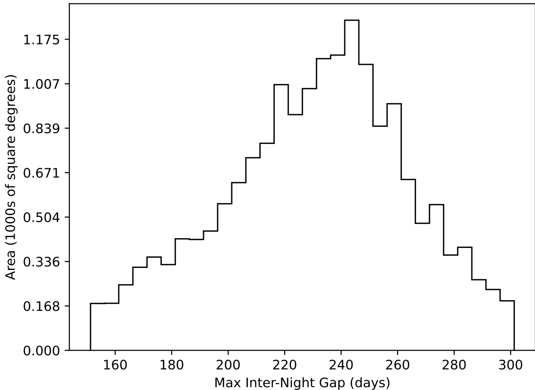
too_elab_r32_d2_gz_v3.4_10yrs WFD all bands: Max Inter-Night Gap
