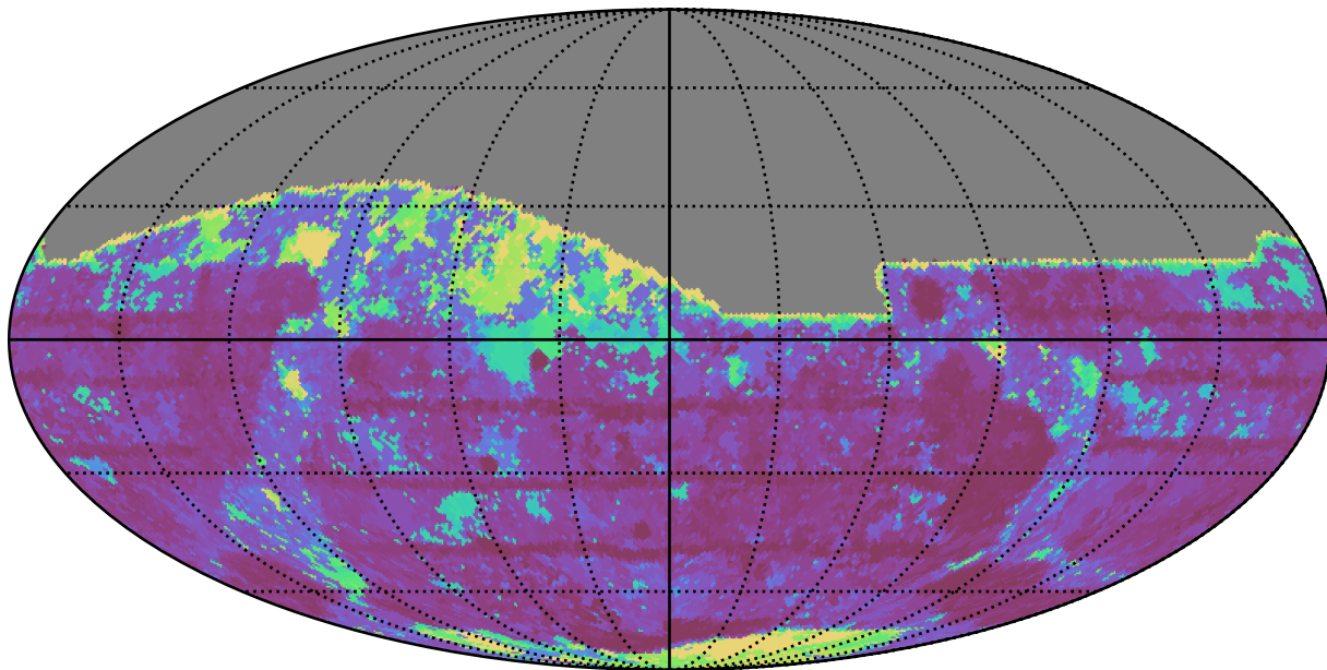
too_elab_r32_d2_gz_v3.4_10yrs All sky z band: Max Inter-Night Gap
