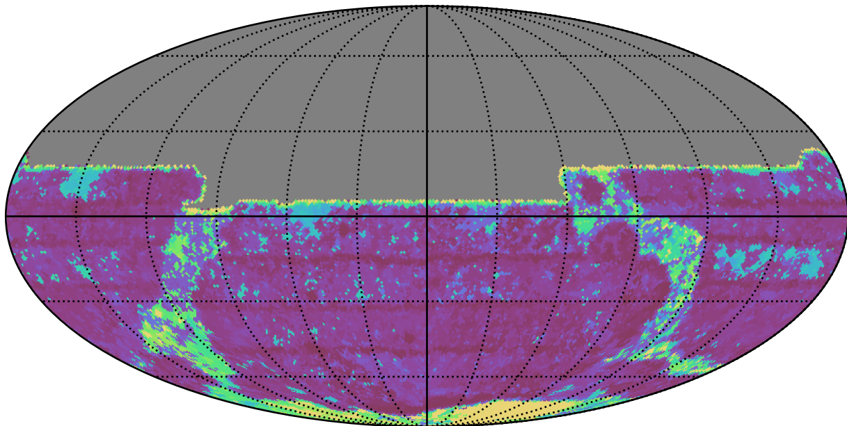
too_elab_r32_d2_gz_v3.4_10yrs All sky y band: Max Inter-Night Gap
