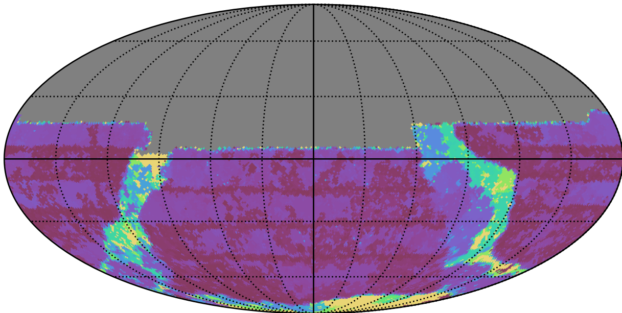
too_elab_r32_d2_gz_v3.4_10yrs All sky u band: Max Inter-Night Gap
