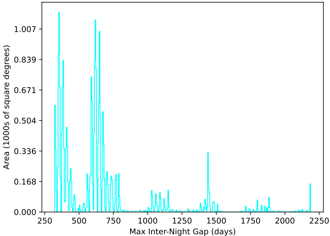
too_elab_r32_d2_gz_v3.4_10yrs All sky u band: Max Inter-Night Gap
