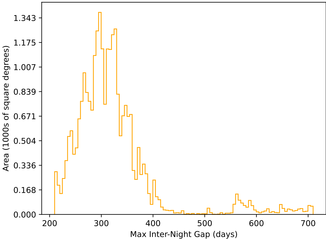
too_elab_r32_d2_gz_v3.4_10yrs All sky r band: Max Inter-Night Gap
