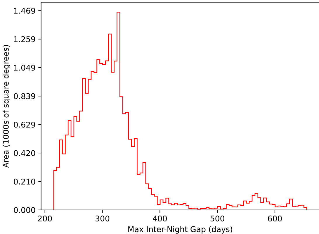
too_elab_r32_d2_gz_v3.4_10yrs All sky i band: Max Inter-Night Gap
