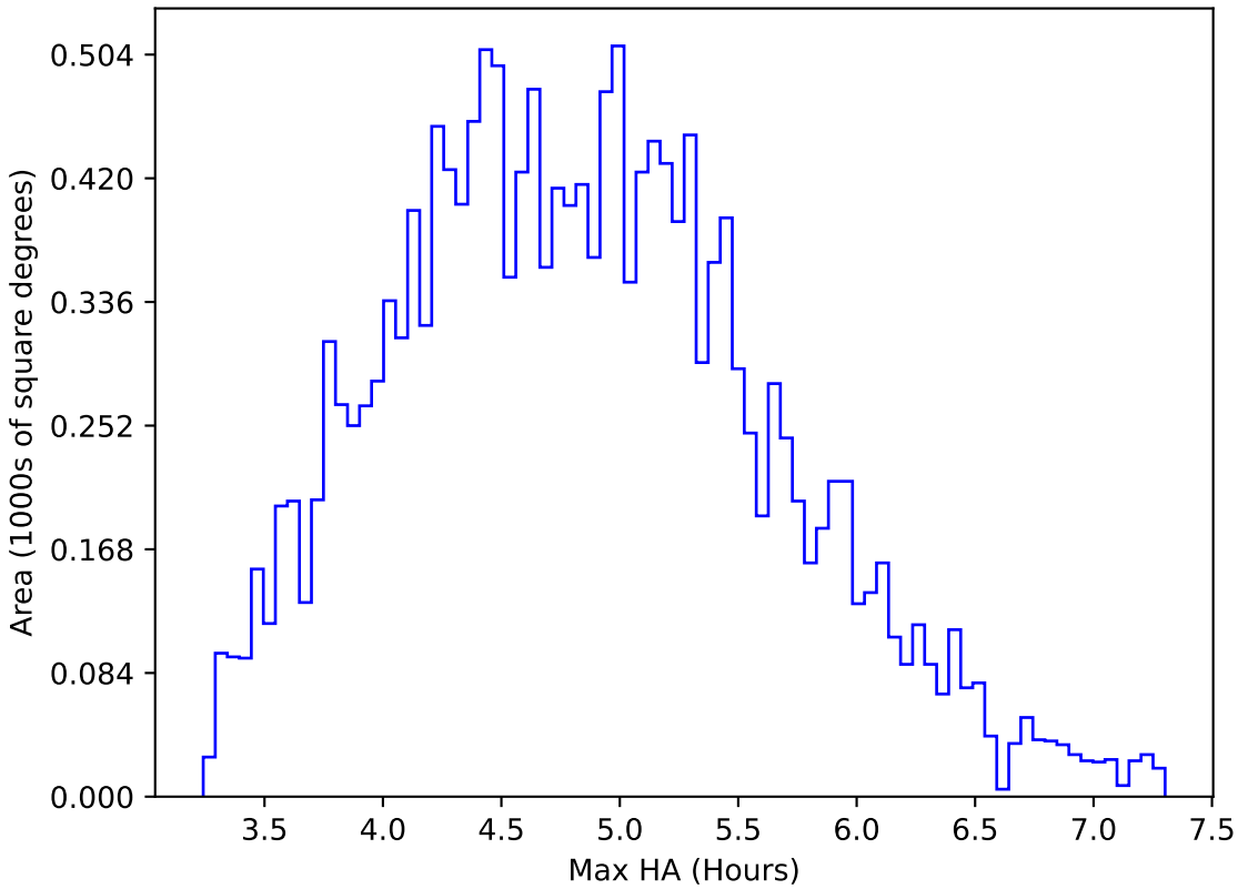
too_elab_r32_d2_gz_v3.4_10yrs WFD z band: Max HA
