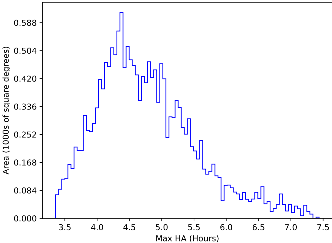
too_elab_r32_d2_gz_v3.4_10yrs WFD y band: Max HA
