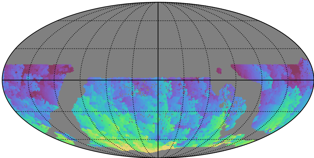
too_elab_r32_d2_gz_v3.4_10yrs WFD u band: Max HA
