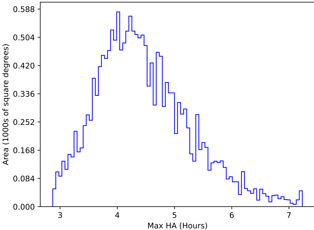
too_elab_r32_d2_gz_v3.4_10yrs WFD r band: Max HA
