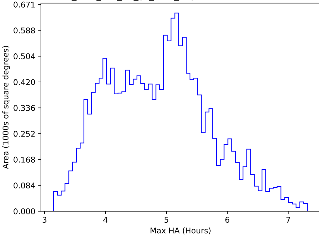
too_elab_r32_d2_gz_v3.4_10yrs WFD i band: Max HA
