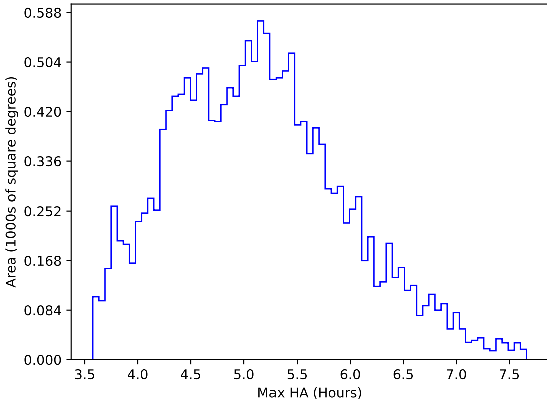
too_elab_r32_d2_gz_v3.4_10yrs WFD all bands: Max HA
