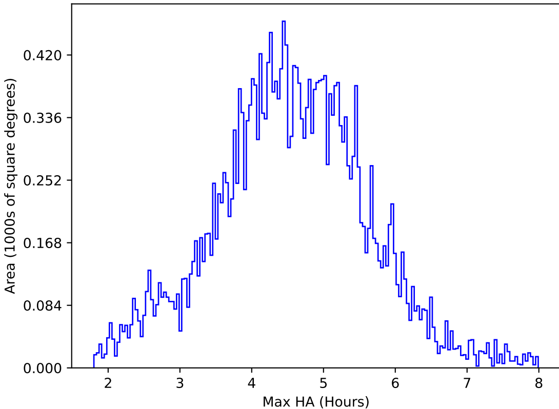
too_elab_r32_d2_gz_v3.4_10yrs All sky z band: Max HA
