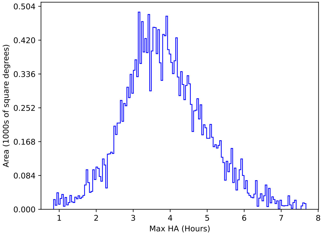
too_elab_r32_d2_gz_v3.4_10yrs All sky u band: Max HA
