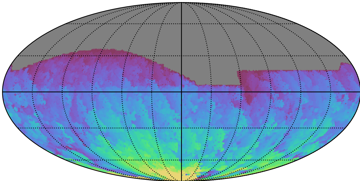
too_elab_r32_d2_gz_v3.4_10yrs All sky r band: Max HA
