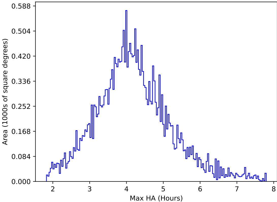
too_elab_r32_d2_gz_v3.4_10yrs All sky r band: Max HA
