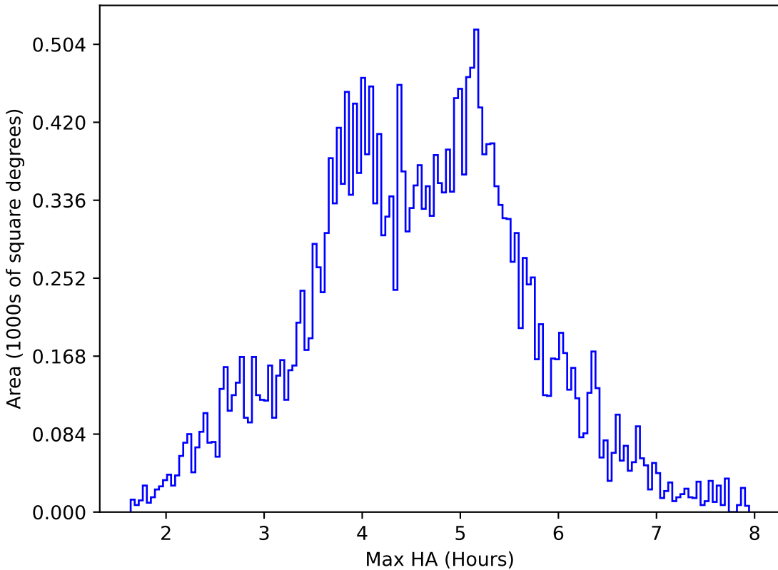
too_elab_r32_d2_gz_v3.4_10yrs All sky i band: Max HA
