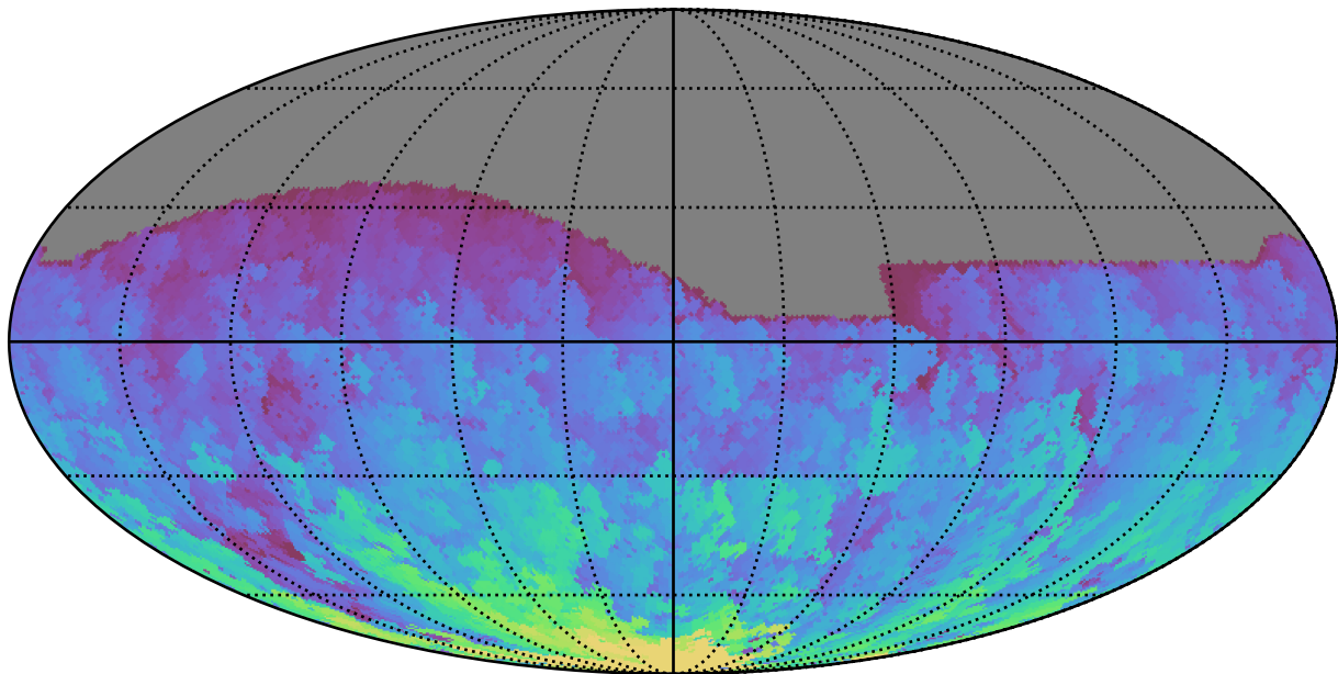
too_elab_r32_d2_gz_v3.4_10yrs All sky g band: Max HA
