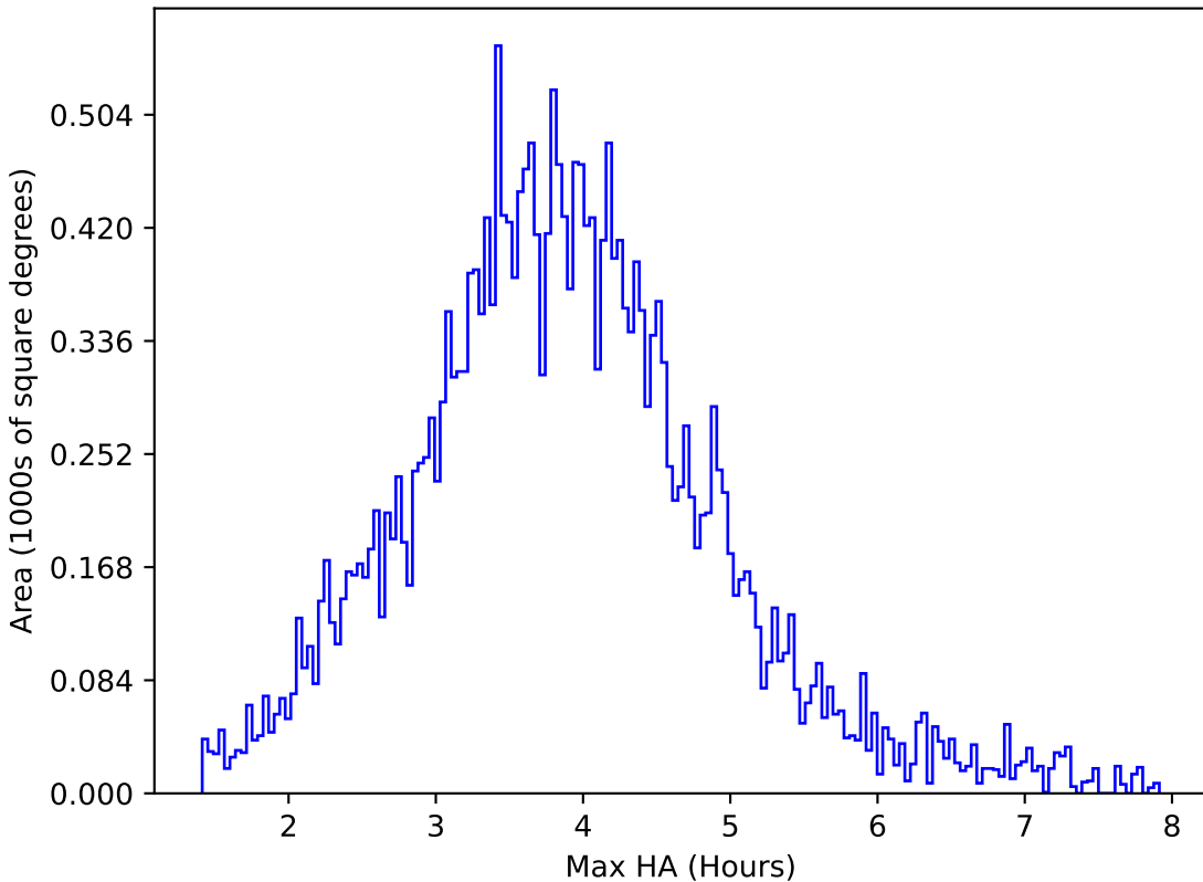
too_elab_r32_d2_gz_v3.4_10yrs All sky g band: Max HA
