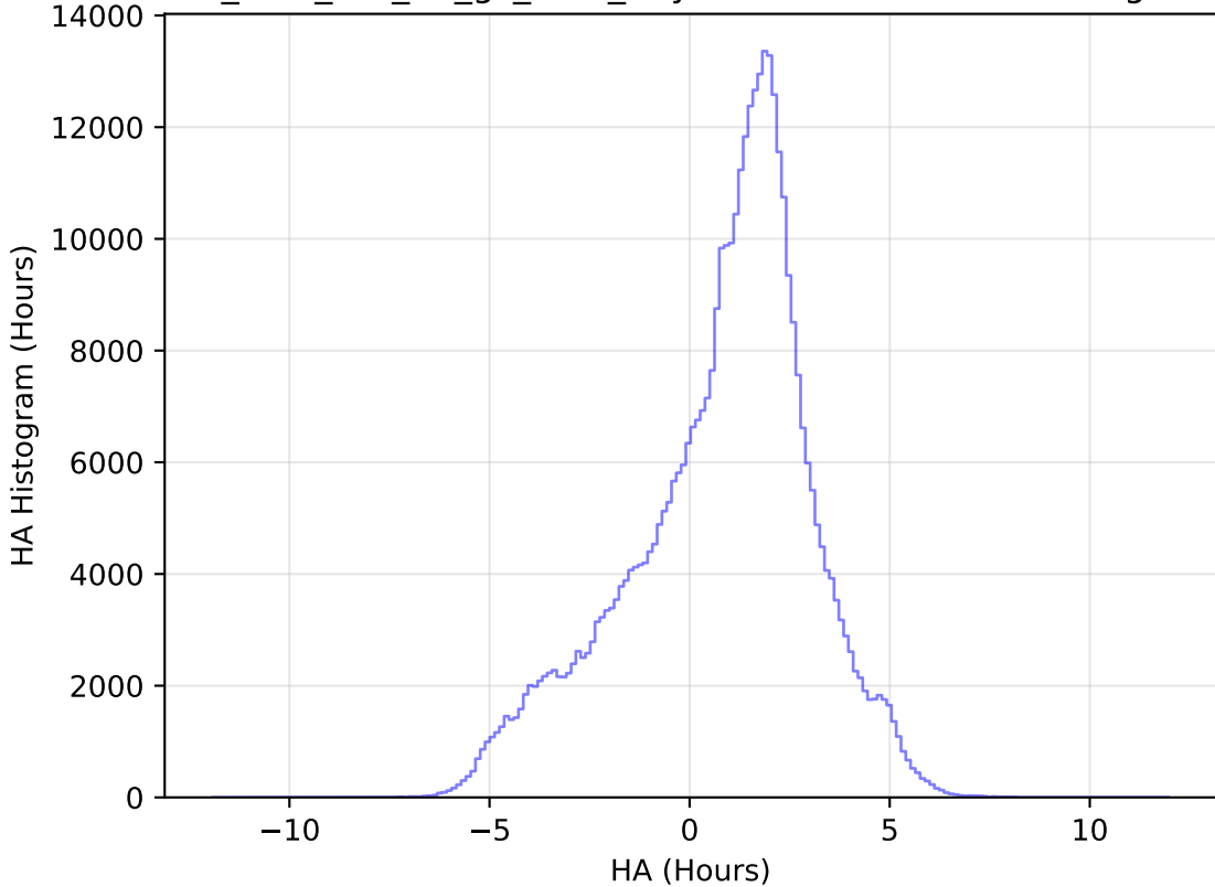
too_elab_r32_d2_gz_v3.4_10yrs WFD z band: HA Histogram
