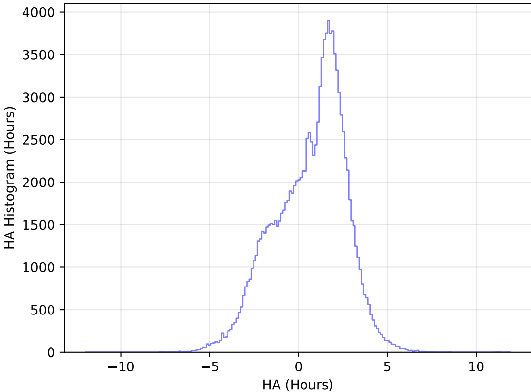
too_elab_r32_d2_gz_v3.4_10yrs WFD u band: HA Histogram
