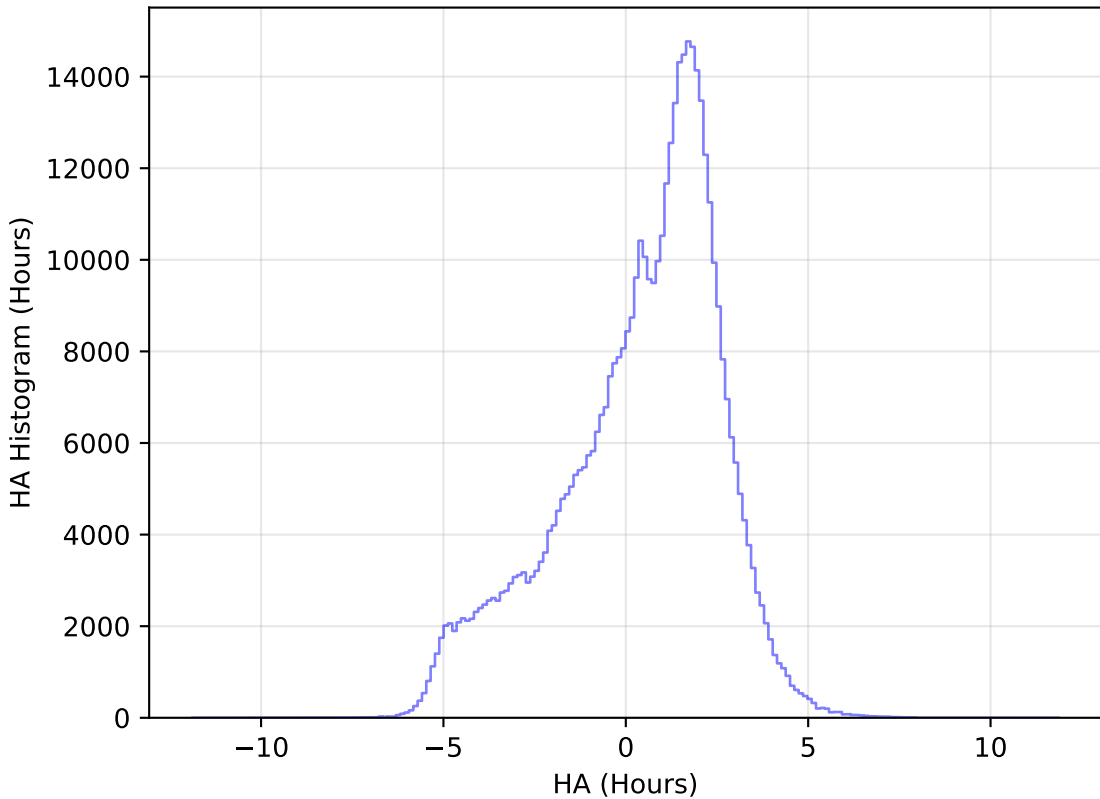
too_elab_r32_d2_gz_v3.4_10yrs WFD r band: HA Histogram
