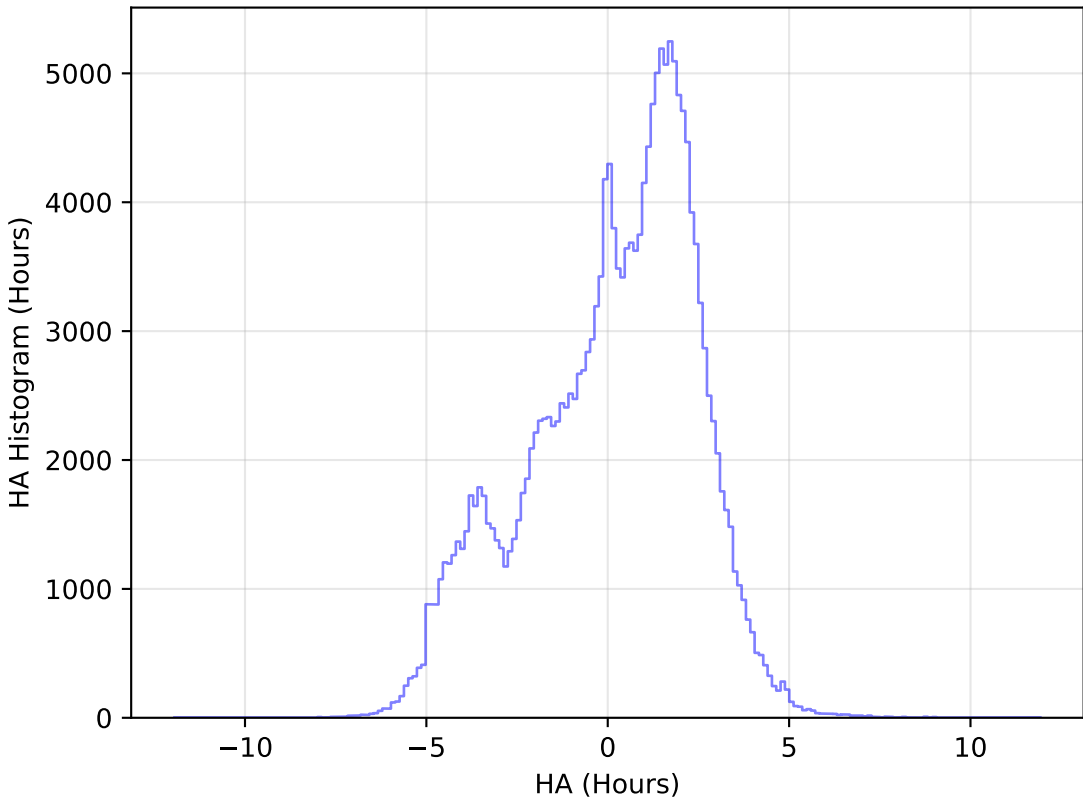
too_elab_r32_d2_gz_v3.4_10yrs WFD g band: HA Histogram
