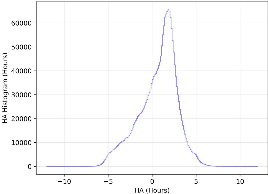
too_elab_r32_d2_gz_v3.4_10yrs WFD all bands: HA Histogram
