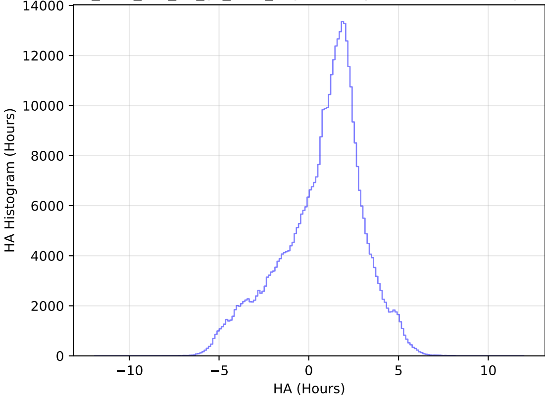
too_elab_r32_d2_gz_v3.4_10yrs All sky z band: HA Histogram
