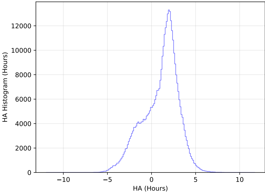
too_elab_r32_d2_gz_v3.4_10yrs All sky y band: HA Histogram
