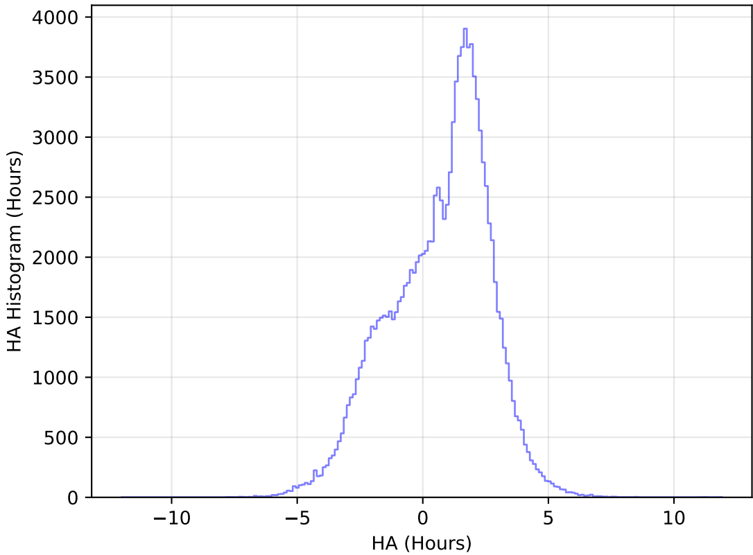
too_elab_r32_d2_gz_v3.4_10yrs All sky u band: HA Histogram
