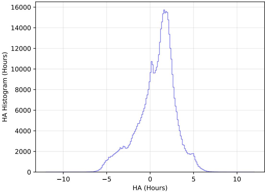
too_elab_r32_d2_gz_v3.4_10yrs All sky i band: HA Histogram
