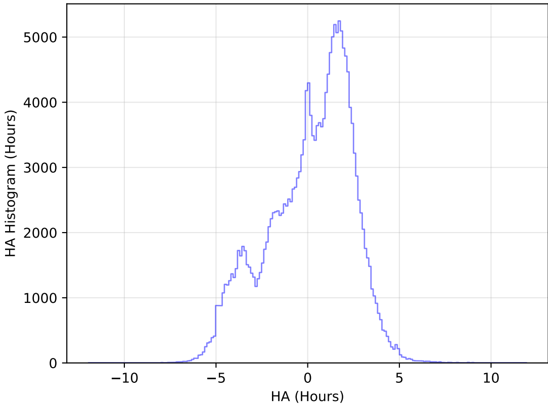
too_elab_r32_d2_gz_v3.4_10yrs All sky g band: HA Histogram
