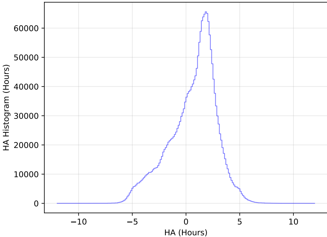
too_elab_r32_d2_gz_v3.4_10yrs All sky all bands: HA Histogram
