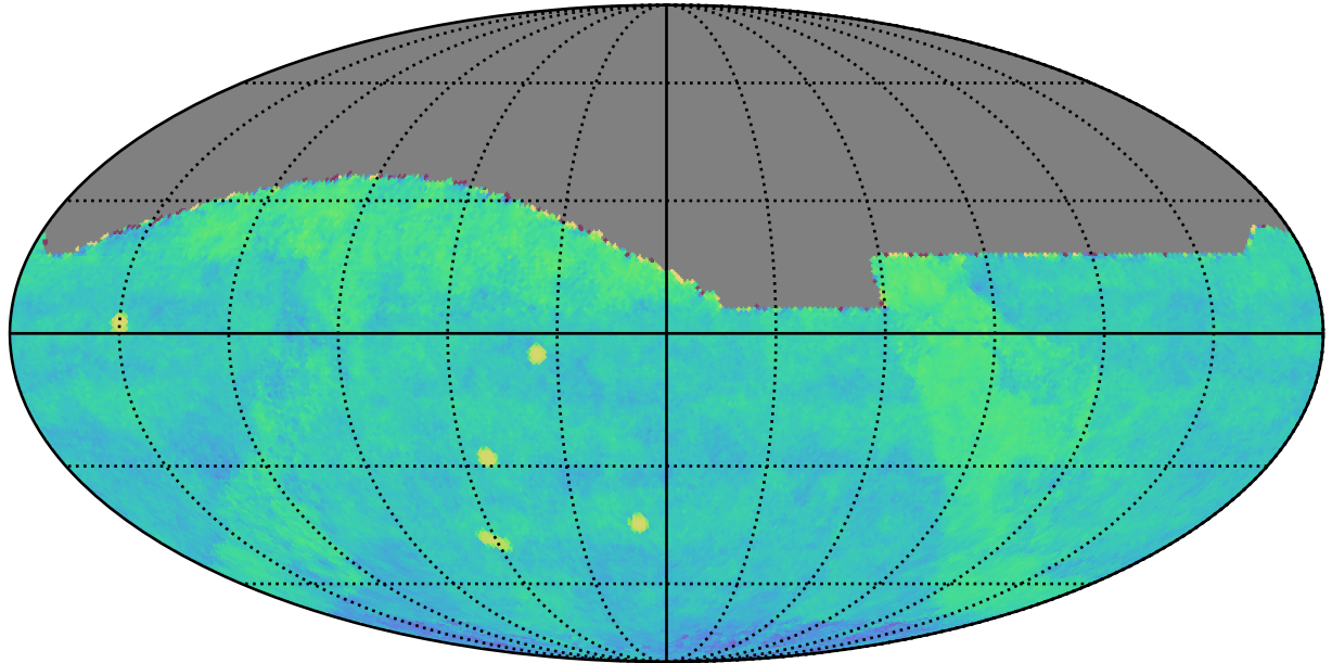
too_elab_r32_d2_gz_v3.4_10yrs gri All sky: Fraction of visits in pairs (10-60 min)
