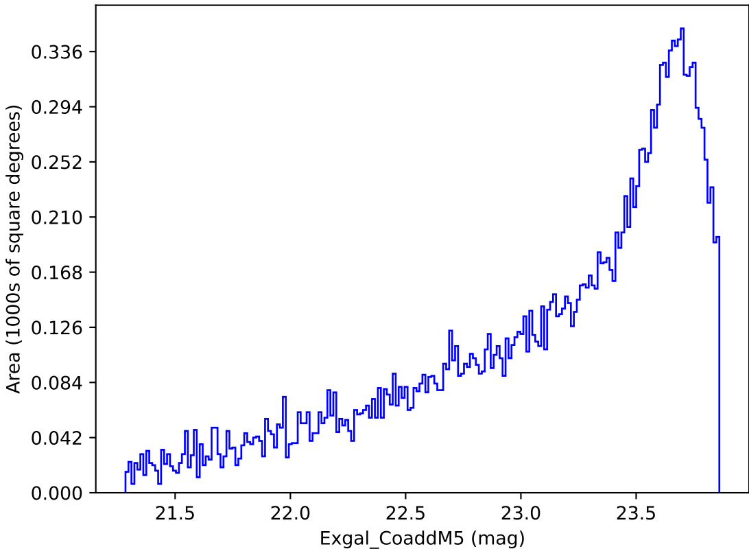
too_elab_r32_d2_gz_v3.4_10yrs Yr 3-4 y band: Exgal_CoaddM5
