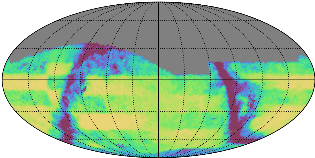
too_elab_r32_d2_gz_v3.4_10yrs Yr 3-4 r band: Exgal_CoaddM5
