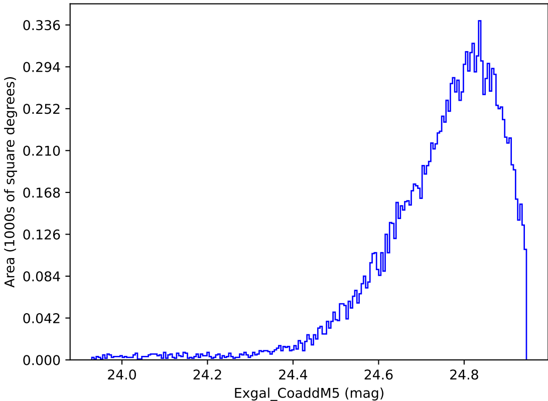
too_elab_r32_d2_gz_v3.4_10yrs WFD y band: Exgal_CoaddM5
