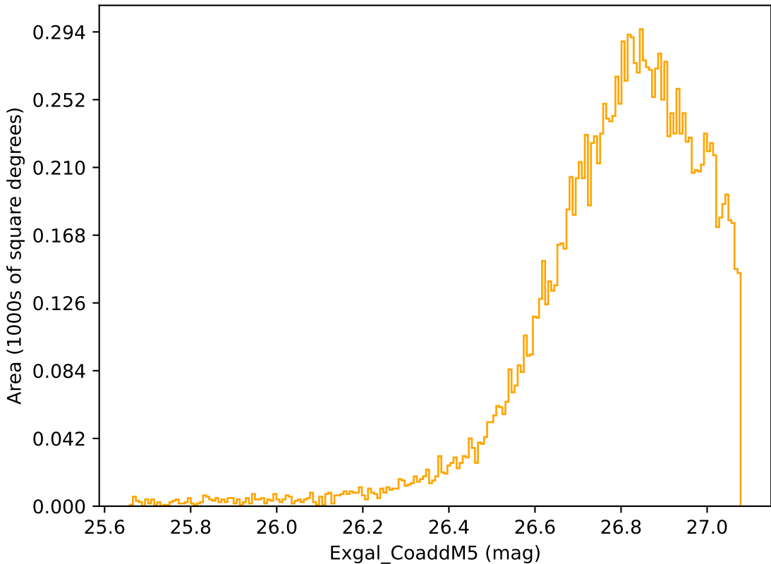
too_elab_r32_d2_gz_v3.4_10yrs WFD r band: Exgal_CoaddM5
