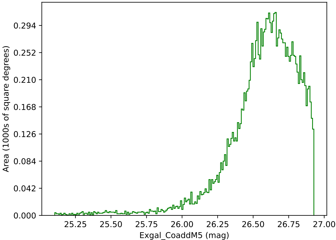
too_elab_r32_d2_gz_v3.4_10yrs WFD g band: Exgal_CoaddM5
