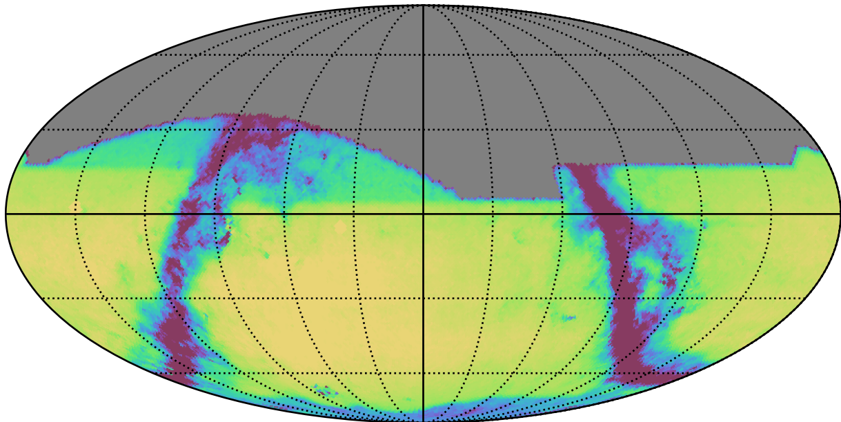
too_elab_r32_d2_gz_v3.4_10yrs All sky r band: Exgal_CoaddM5
