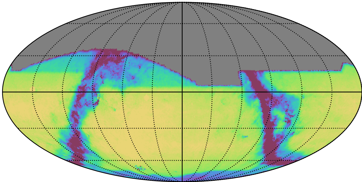
too_elab_r32_d2_gz_v3.4_10yrs All sky i band: Exgal_CoaddM5
