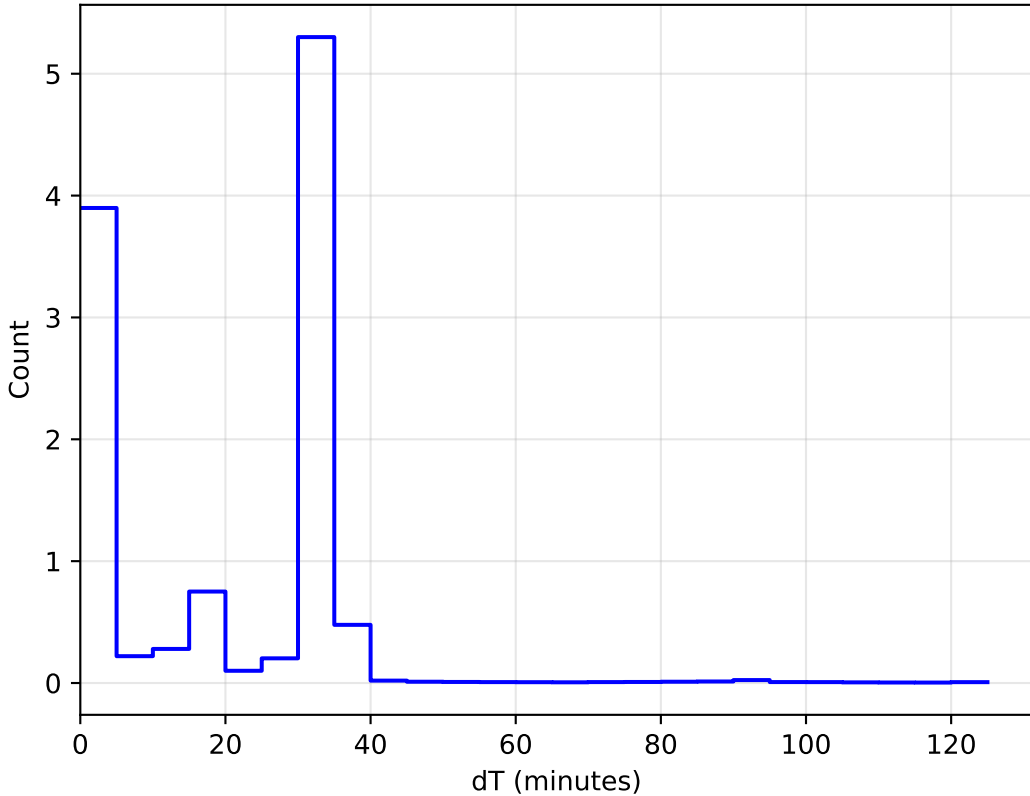
too_elab_r32_d2_gz_v3.4_10yrs WFD: DeltaT Histogram
